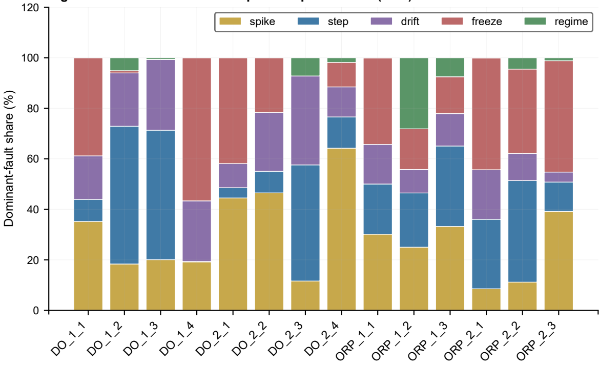
Figure 6. Dominant fault decomposition per channel (final)
